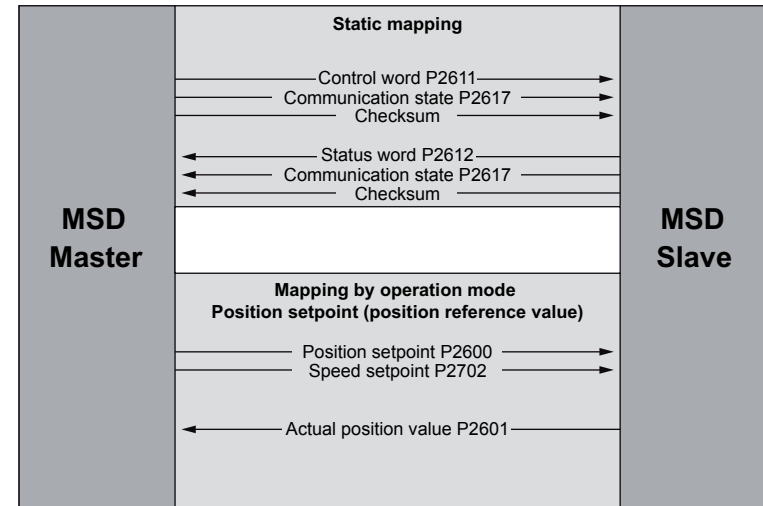
Figure 5.12: Process data interface, position setpoint (position reference value)
