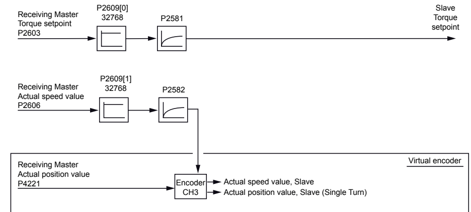
Figure 5.11: Virtual encoder VE (torque) control structure
