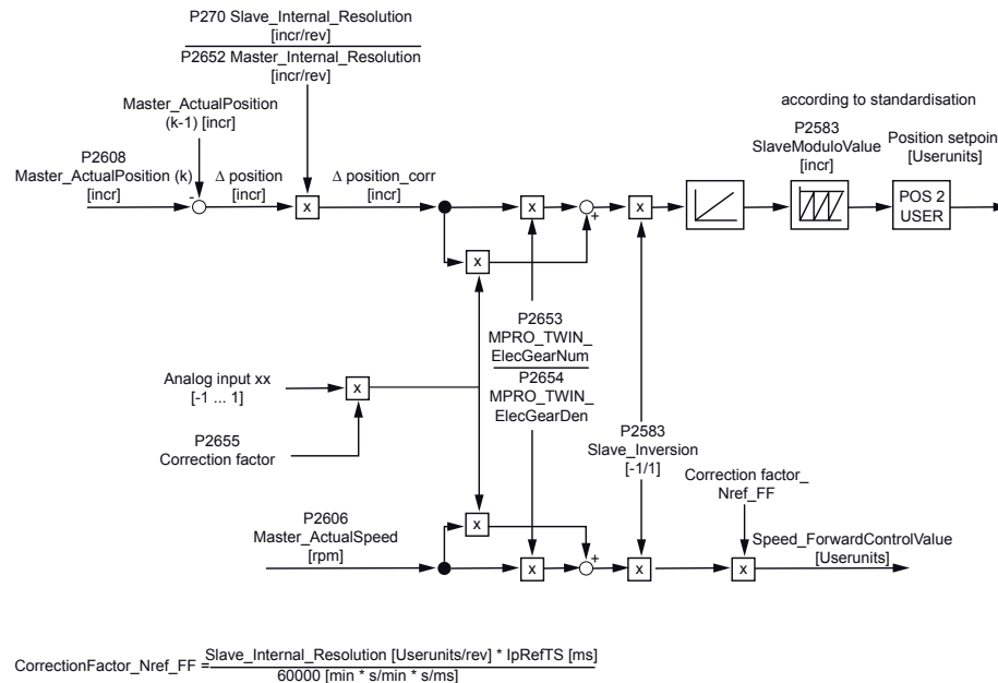
Figure 5.7: Control structure for position control (TWINpos)
