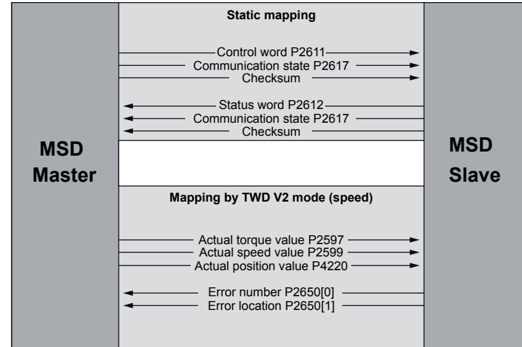
Figure 5.3: Process data interface between the master and slave drives in the operation mode: "TWin-Drive-Profile TWD" (speed) Version 2
