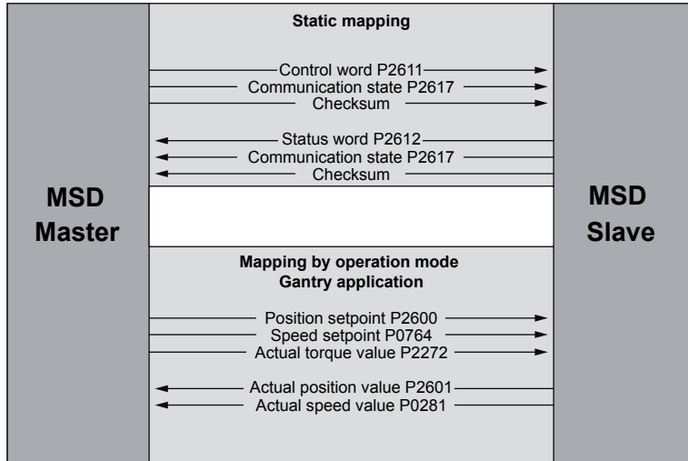
Figure 5.13: Process data interface, gantry application
