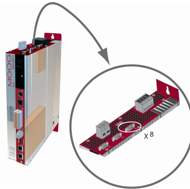
Figure 1.1: The TWINsync option for TWINsync coupling of two MSD Servo Drives
