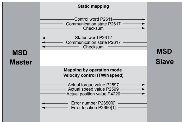
Figure 5.5: Process data interface between the master and slave drives in the operation mode: Speed control (TWINspeed)
