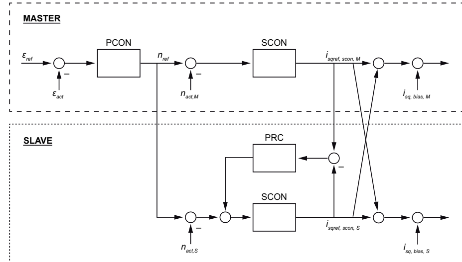
Figure 5.9: "Rack and pinion drive control RPDC" control structure
