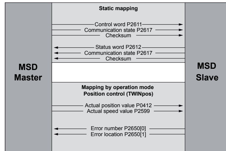
Figure 5.6: Process data interface between the master and slave drives in the operation mode: Position control (TWINpos)
