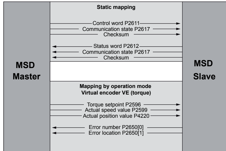
Figure 5.10: Process data interface between the master and slave drives in the operation mode: "Virtual Encoder VE" (torque)
