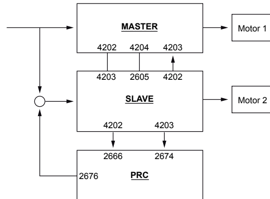
Figure 5.8: Process data interface and process controller "Rack and pinion drive control RPDC"
