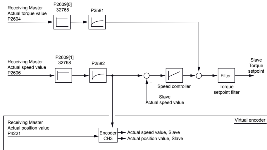
Figure 5.4: Control structure for "TWIn-Drive-Profile TWD" (speed) Version 2
