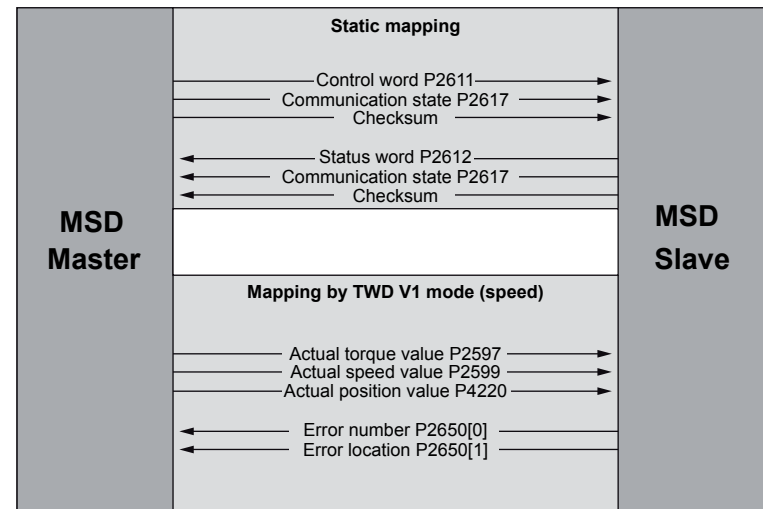
Figure 5.1: Process data interface between the master and slave drives in the operation mode: "TWin-Drive-Profile TWD" (speed) Version 1
