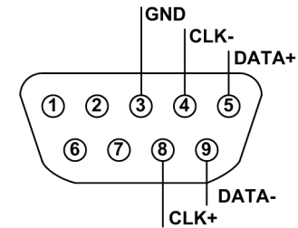
Figure 1.1 Pin assignment of SSI Encoder Simulation
