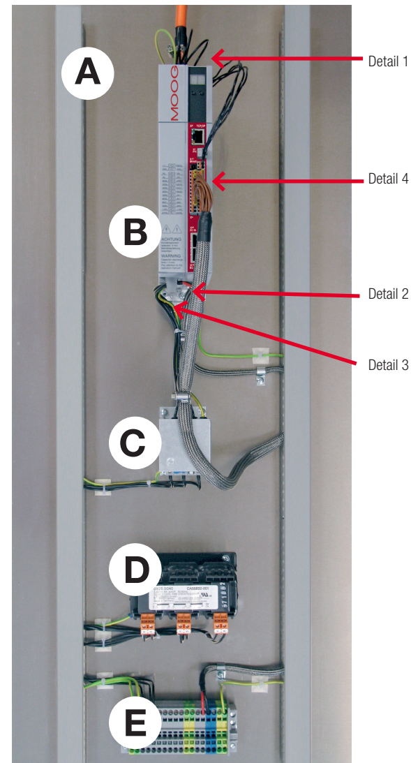
Figure 4.5 Specimen setup - Overview
