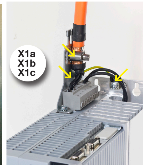
Figure 4.9 Detail 1: Motor cable C5
